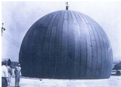
Figure 4 - The first radome prototype (1948). Walter Bird stands on top (Topham, 2002)
