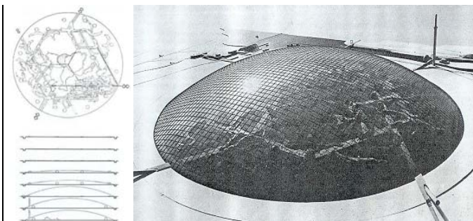
Figure 7: The Arctic City of Frei Otto and Ewald Bubner, 1970. Plan, insulating process and model (Herzog, 1977)
