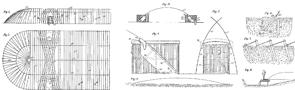
Figure 2: Details of Lanchester's patent for inflated tents (1918) (Herzog, 1977).
